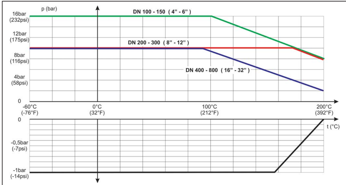
Fig. 7 - Pressure-Temperature diagram
