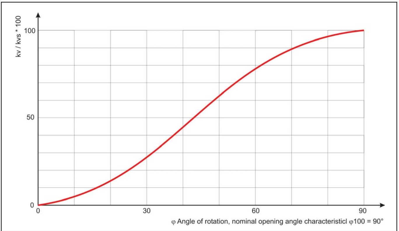
Fig. 6 – Characteristic curve
