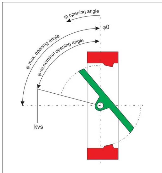
Fig. 8 - Functional diagram with opening angles
