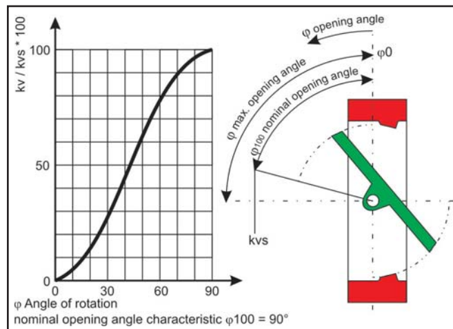
Fig. 6 - characteristic curve and functional diagram with opening angles
