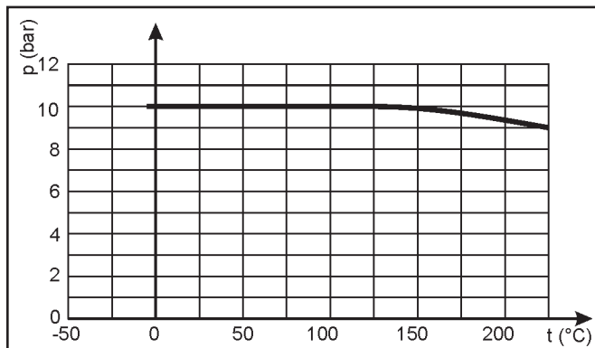
Fig. 5 - pressure-temperature diagram
