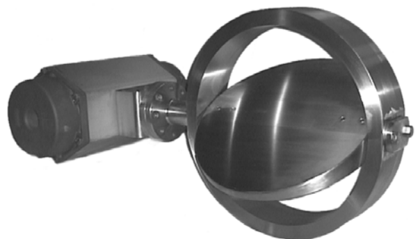
Fig. 2 - Butterfly valve Series 14e with pneumatic rotary actuator Series 31a
