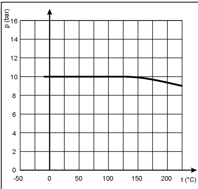
Fig. 4 - pressure-temperature diagram
