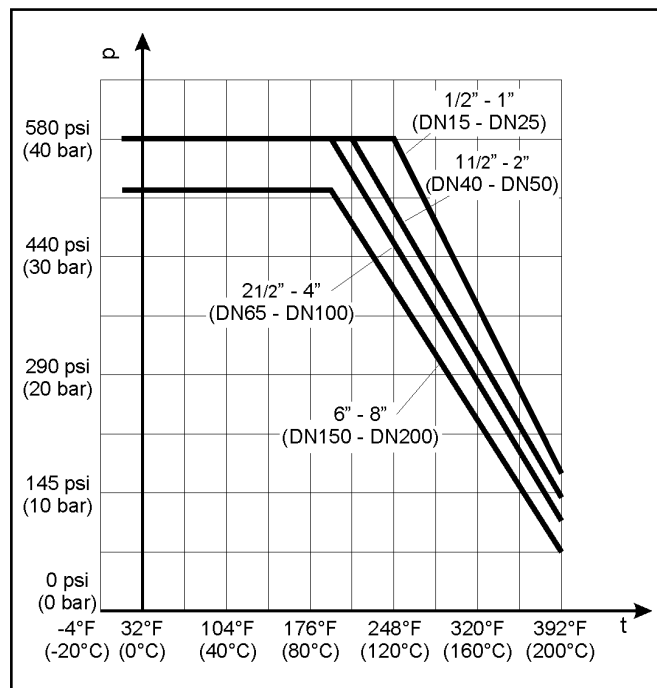
Fig. 6 - Pressure-Temperature diagram
