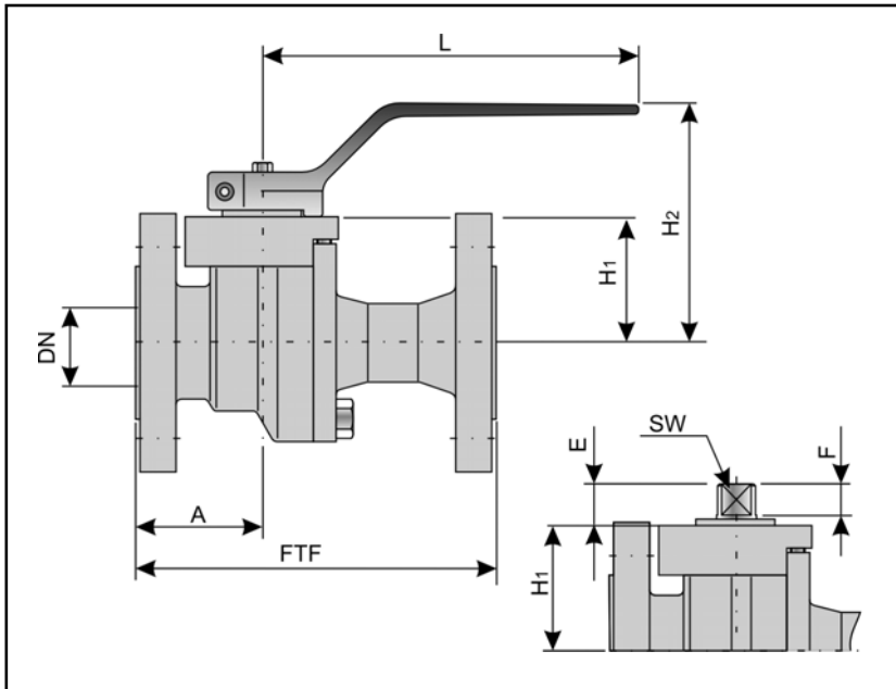
Fig. 7 - Dimensional drawing
