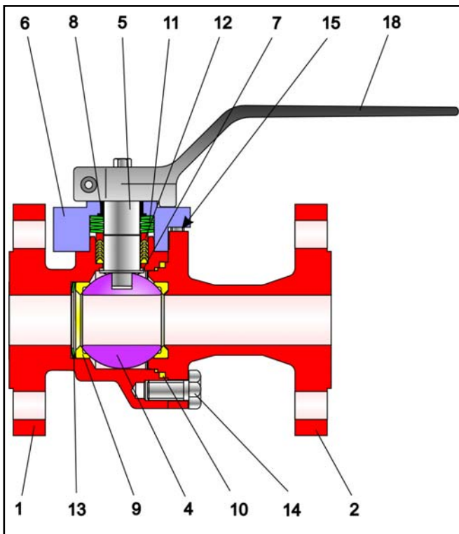
Fig. 3 – Sectional diagram of Series 26a Ball Valve
