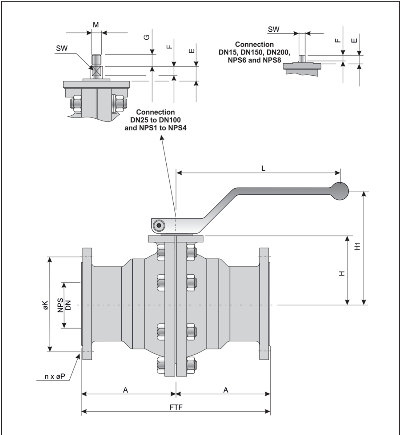
Fig. 8 - Dimensions in mm and weights in kg
