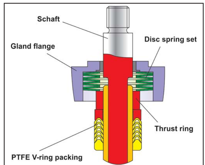
Fig. 5 - Live-loaded sealing system
