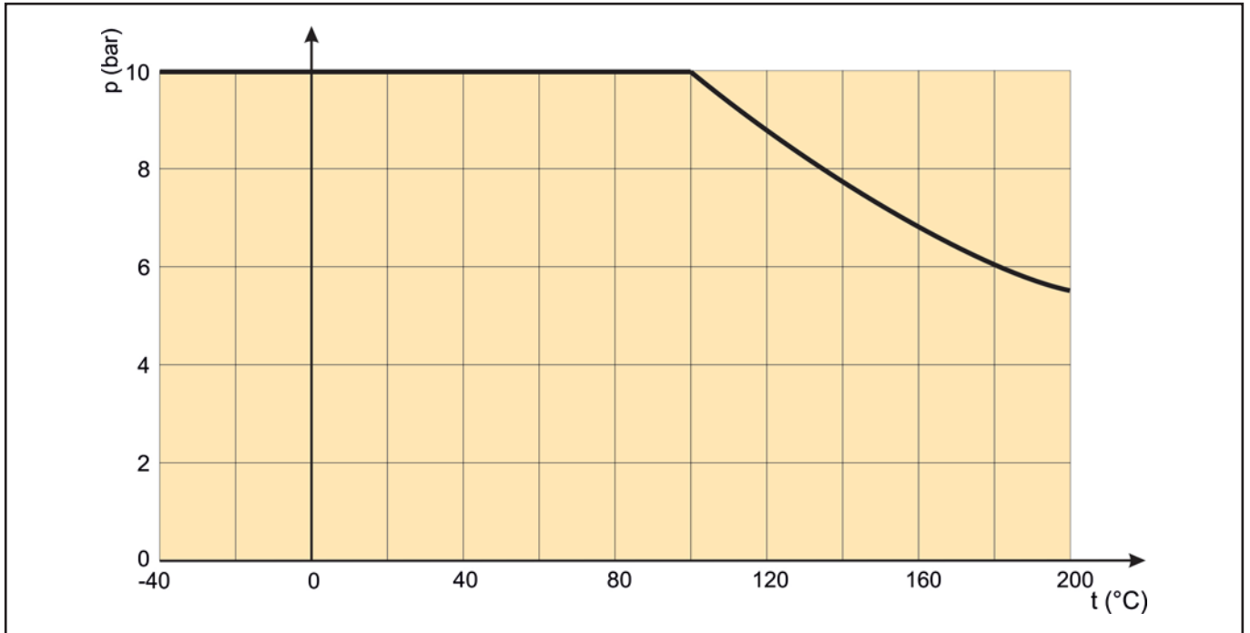
Fig. 5 - Pressure-temperature diagram
