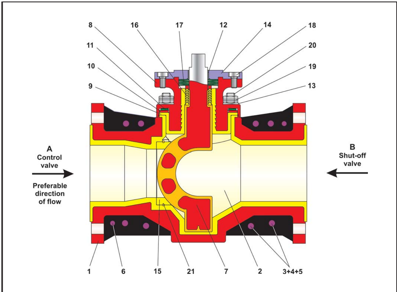
Fig. 2 - BR 23e PTFE-lined Rotary Plug Valve
